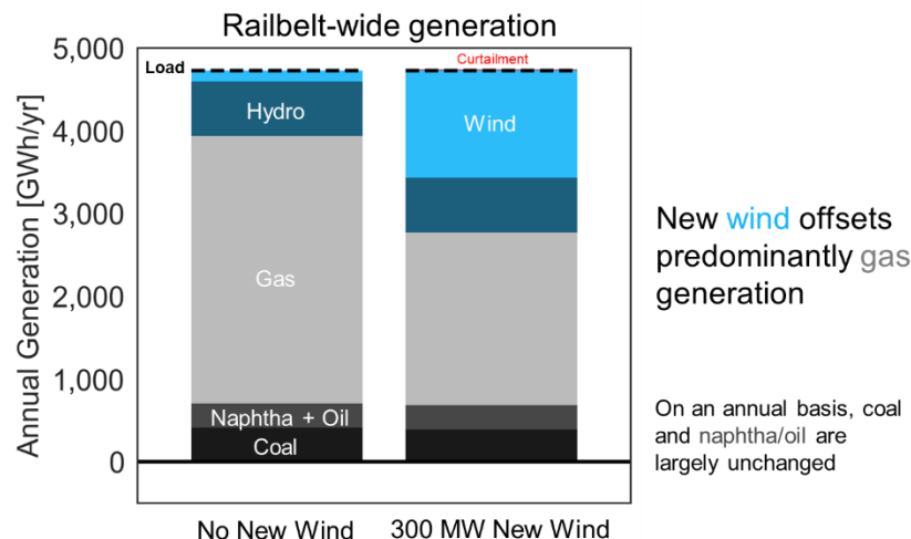
Figure 6: Railbelt-wide annual generation comparison between the No New Wind and 300 MW New Wind Scenarios. The same information broken out by zone is found in Figure 7.
