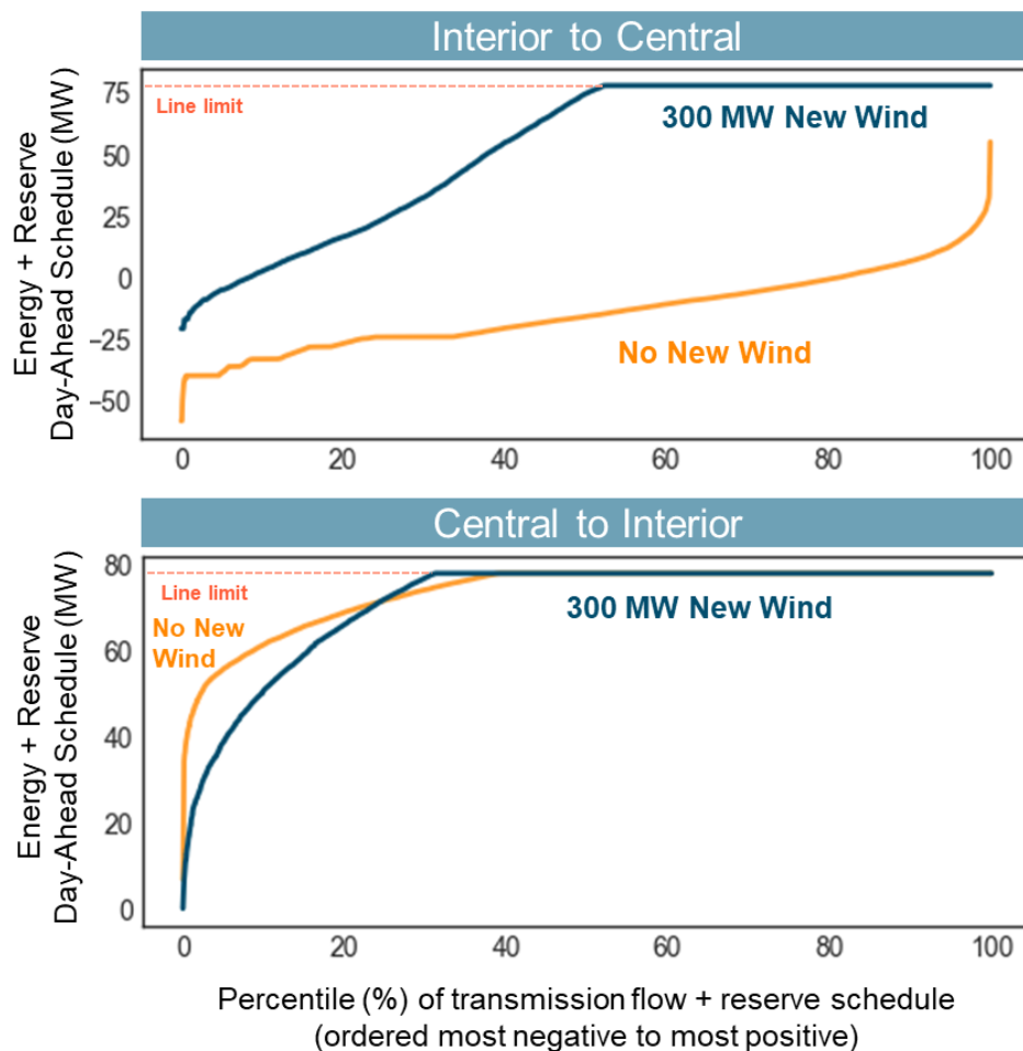
Figure 22: Day-ahead utilization (energy + reserve schedule) of the Alaska Intertie in each direction for both the No New Wind Scenario and the 300 MW New Wind Scenario.
